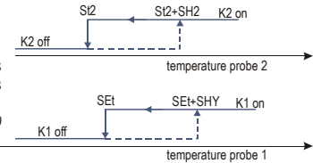
Figure 3: 2 INDEPENDENT STAGES WITH 2 PROBES if Sdb=0, Pr2=1 Example with Act=0 & Ac2=0
