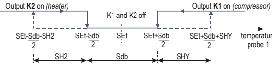
Figure 3: 2 INDEPENDENT STAGES WITH 2 PROBES if Sdb=0, Pr2=1 Example with Act=0 & Ac2=0
