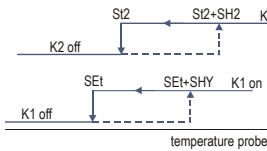
Figure 2: 2 INDEPENDENT STAGES WITH 1 PROBE if Sdb=0, Pr2=0 Example with Act=0 & Ac2=0
